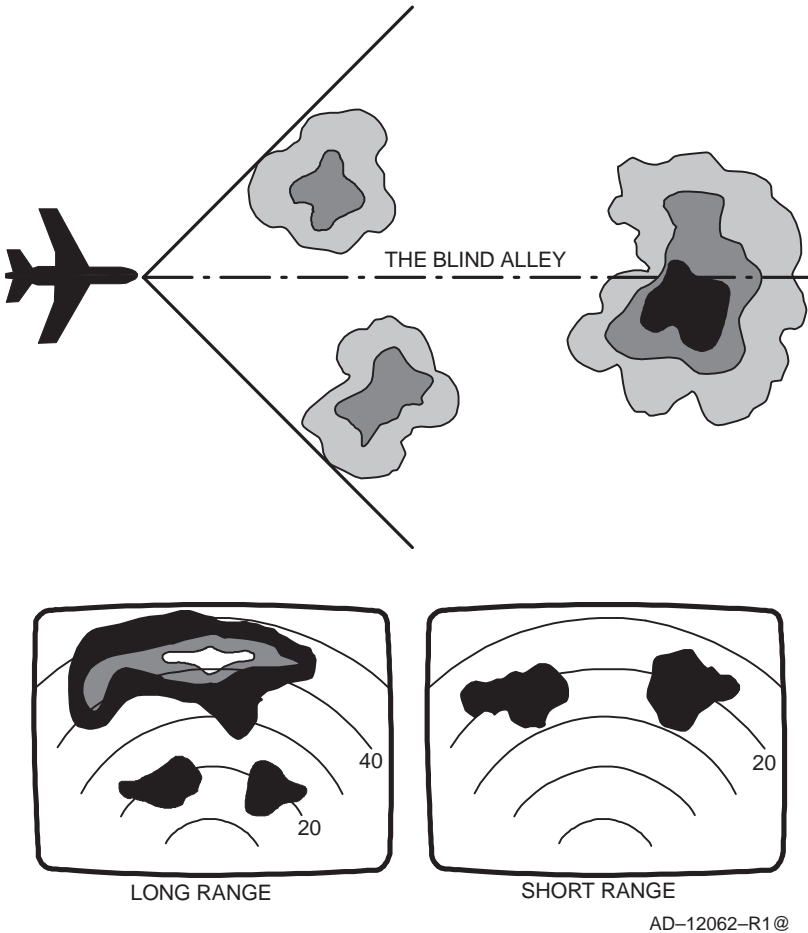
Short- and Long-Blind Alley Figure 5-37
