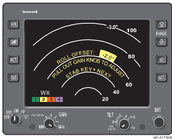
Roll Offset Adjustment Display – Initial Figure 7-4
