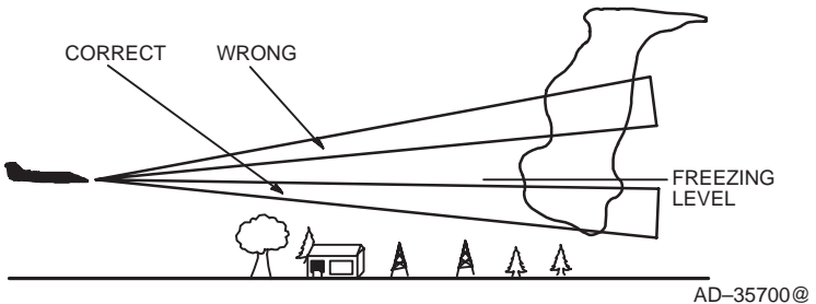
Low Altitude Tilt Management Figure 5–15
