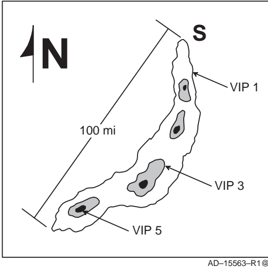
Bow-Shaped Line of Thunderstorms Figure 5-46
