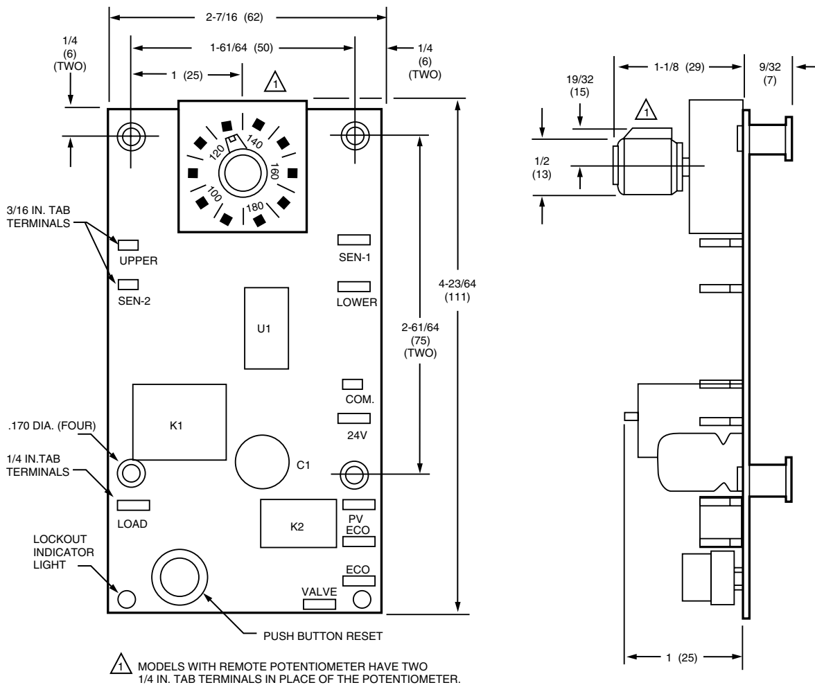
Fig. 3—Approximate dimensions in in. (mm) of L8104C,D Electronic Control Module.
