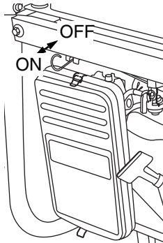
FIGURE 26: Choke Control
