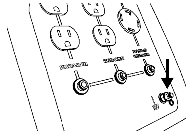
FIGURE 11: Ground Terminal
