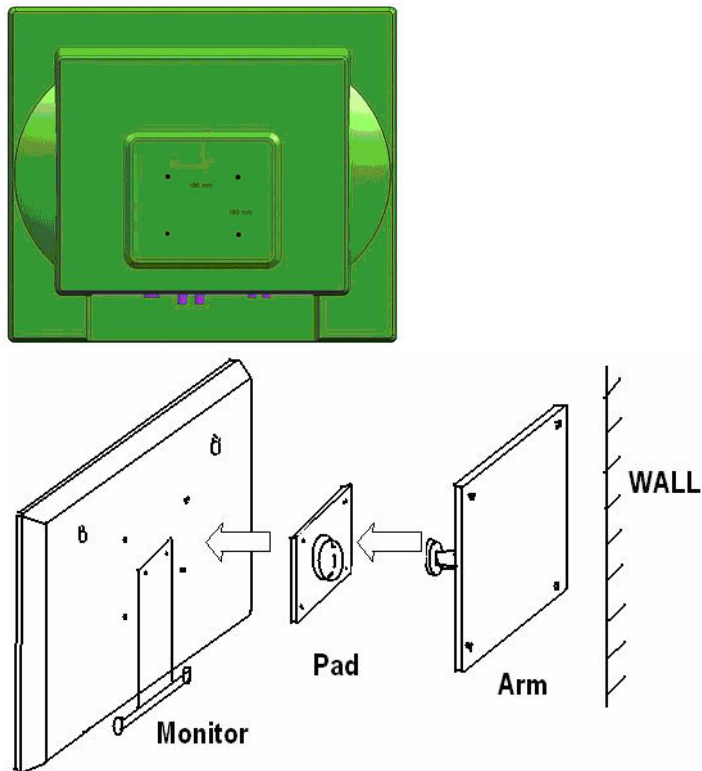
Figure 5 Back of the LCD monitor and mounting
