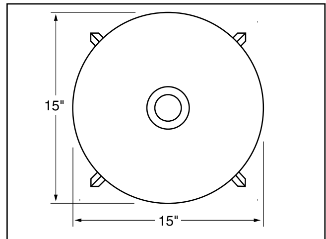
Figure 5. T26417 Minimum working clearances.
