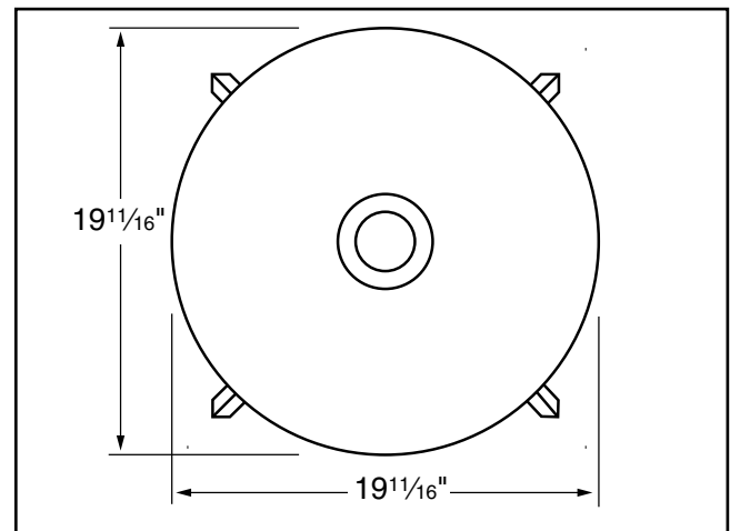
Figure 6. T26418 Minimum working clearances.
