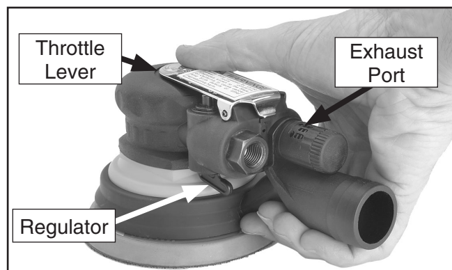
Figure 4. Sander controls.
