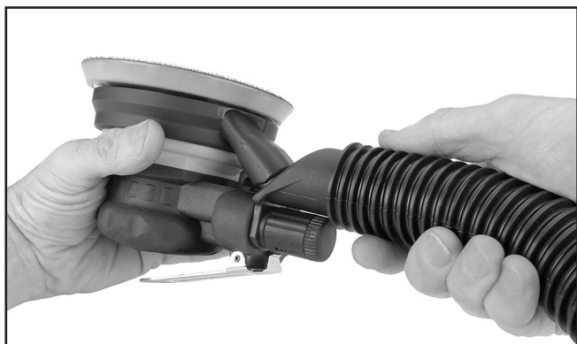
Figure 3. Attaching sander to 1 1/4" canister vacuum hose.
