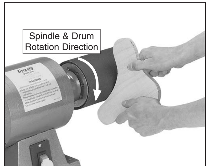
Figure 15. Typical drum sanding operation.
