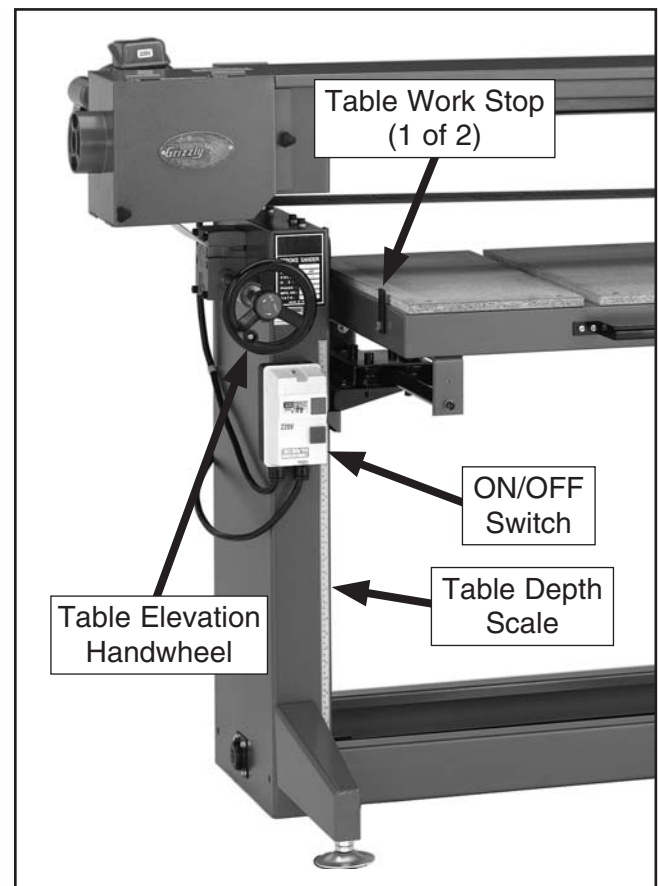
Figure 31. Basic controls.
