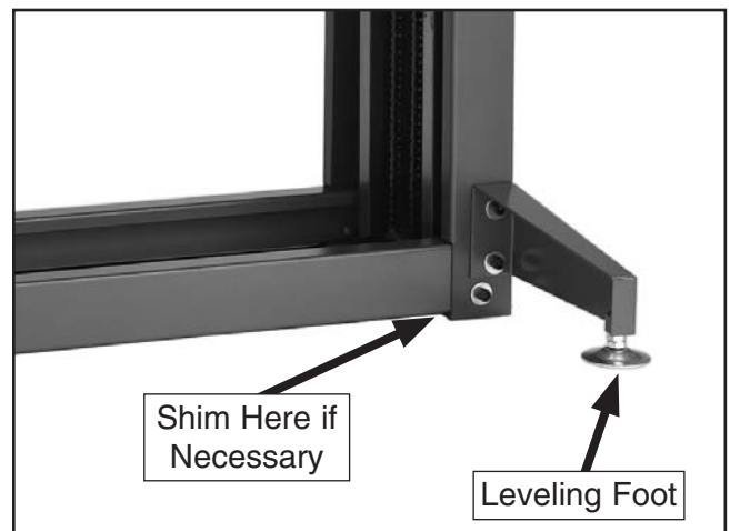
Figure 29. Machine leveling.
