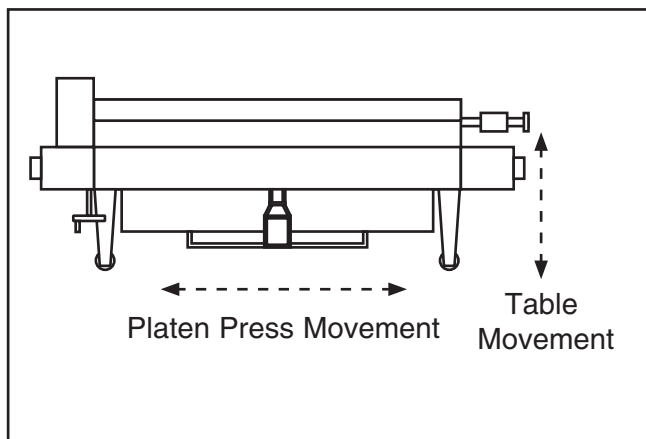
Figure 38. Sanding movements.
