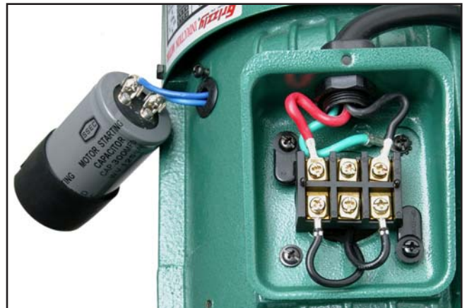
Figure 52. Motor wiring.
