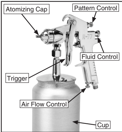
Figure 3. Controls.
