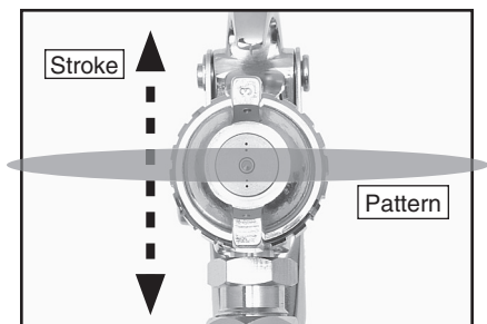
Figure 7. Set up for vertical stroke direction with horizontal fan pattern.
