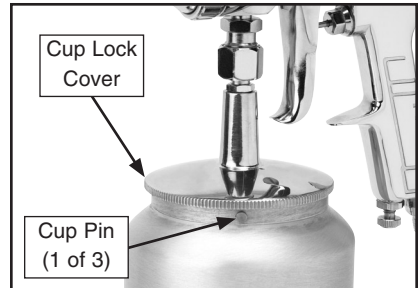
Figure 4. Installing cup.
