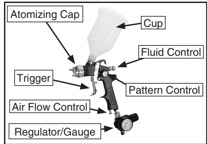
Figure 3. Controls.
