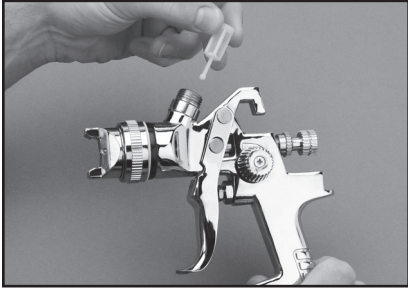
Figure 3. Installing filter.
