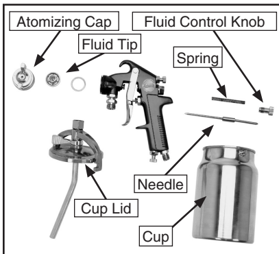
Figure 14. Disassembly for cleaning.
