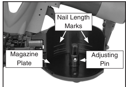
Figure 4. Positioning the magazine plate.
