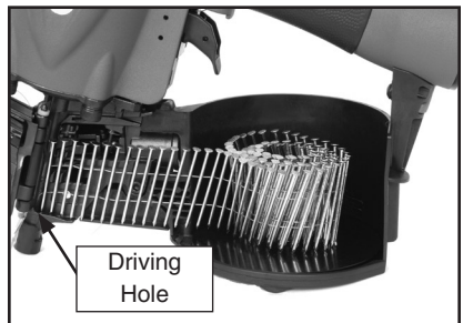
Figure 5. Loading nails in the magazine.
