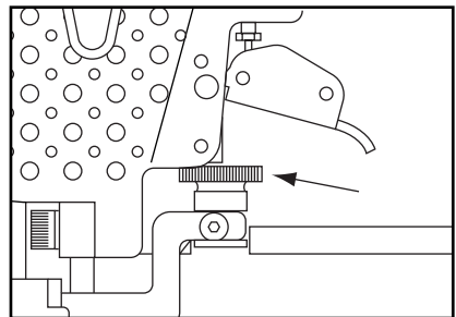
Figure 6. Depth adjustment wheel.
