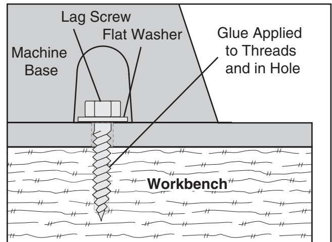
Figure 9. Surface mount using lag screws.
