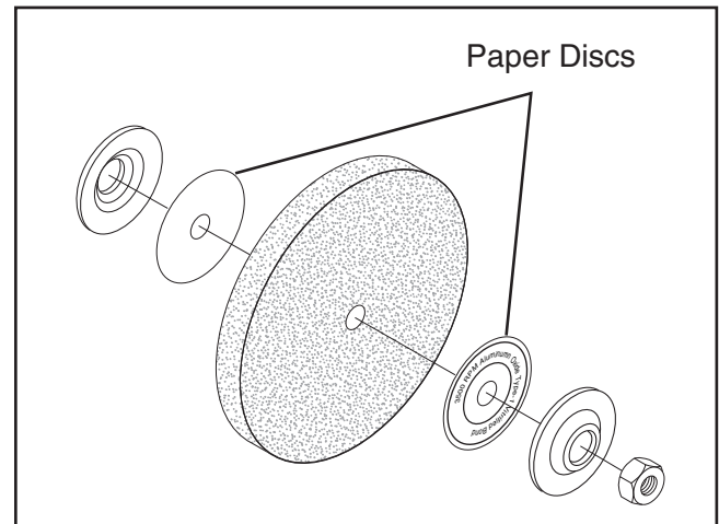
Figure 17. Assembly order for wheel installation.
