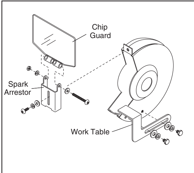
Figure 10. Model T24463 spark deflector, safety shield, and tool rest installation.
