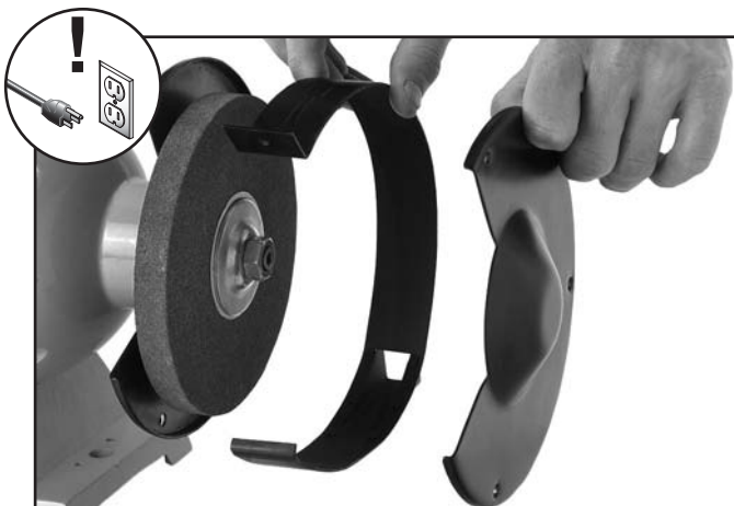
Figure 16. Model T24464 wheel guard components.
