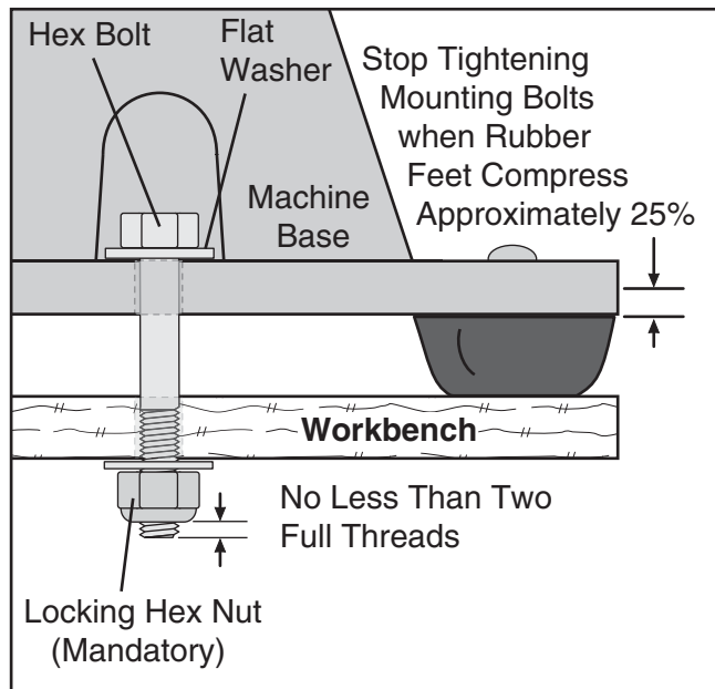
Figure 7. "Through Mount" with rubber feet installed.
