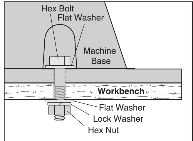
Figure 8. Through mount using nuts and bolts.
