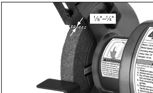
Figure 11. Spark deflector gap.
