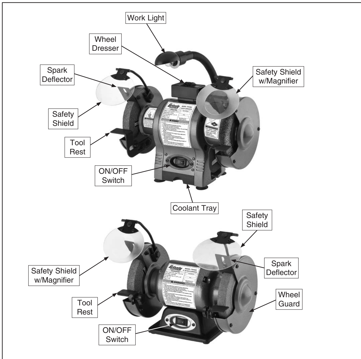
Figure 2. Machine identification.
