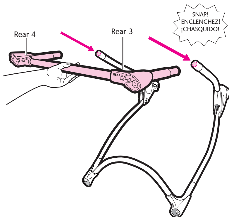
Rear tube Tube arrière Tubo trasero
