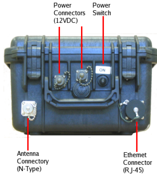
Figure 3-4. BreadCrumb XL - External Connector
