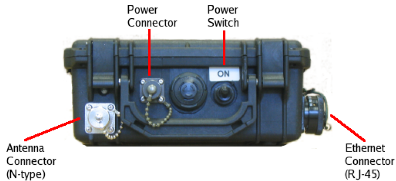
Figure 3-3. BreadCrumb SE - External Connectors
