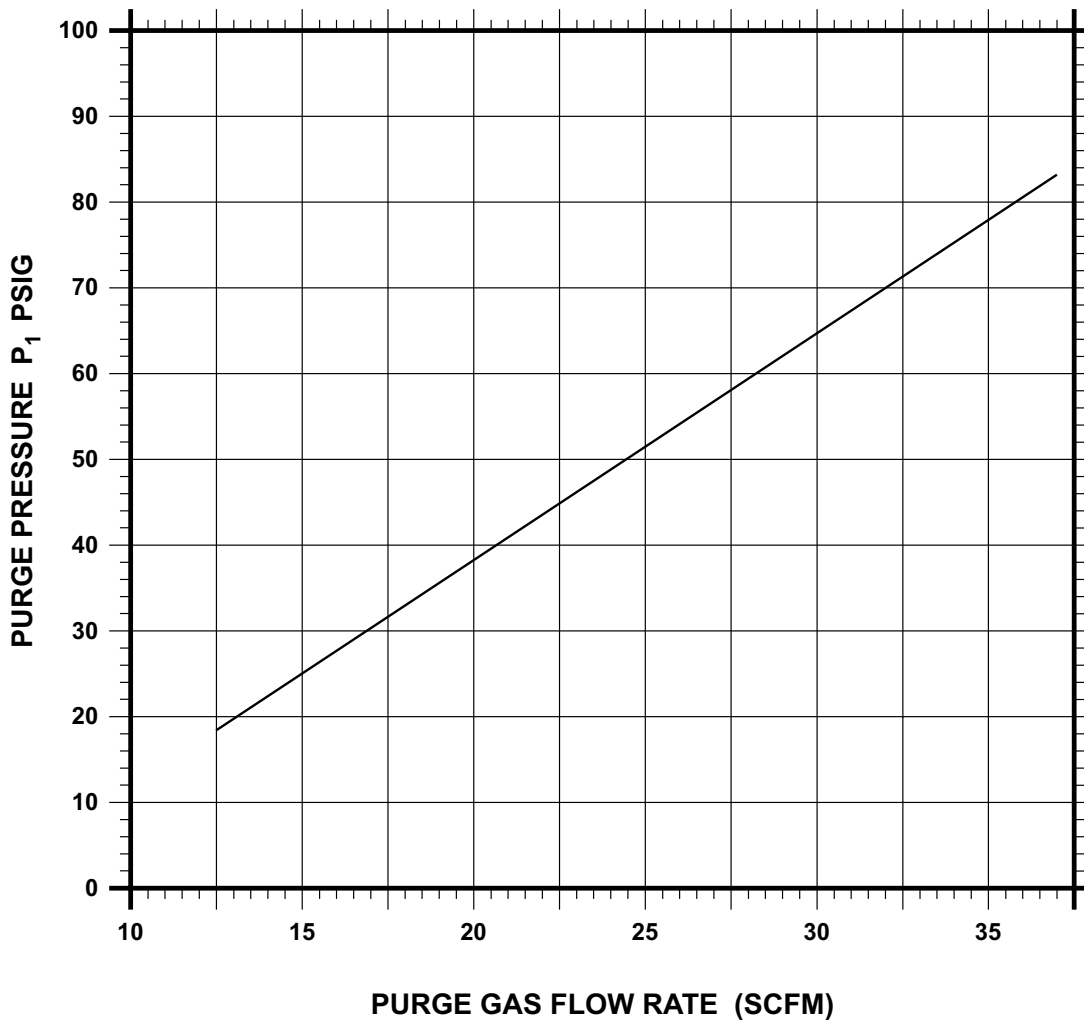
Figure C.5 — Critical Orifice Calibration Curve (LSC240, LSC270)
