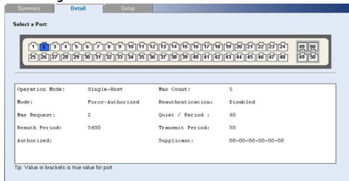
Figure 58 802.1X Detail Screen
