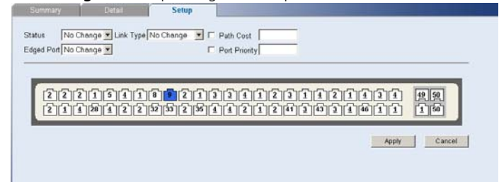
Figure 47 Spanning Tree Setup Screen
