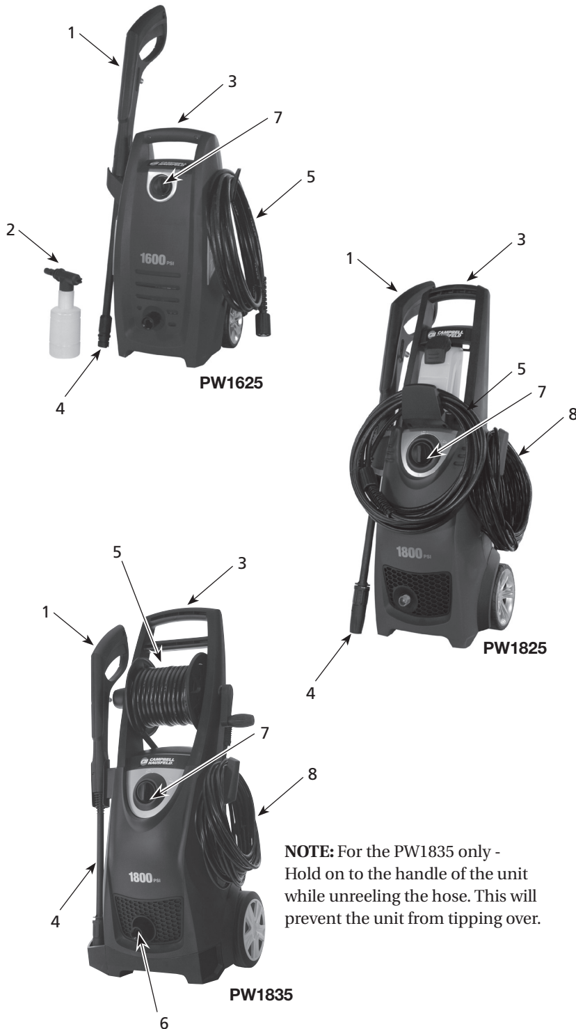
Figure 6 - Components of the Pressure Washer
