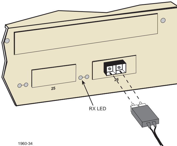
Figure 3-11 FE-100FX and FE-100F3 Ports
