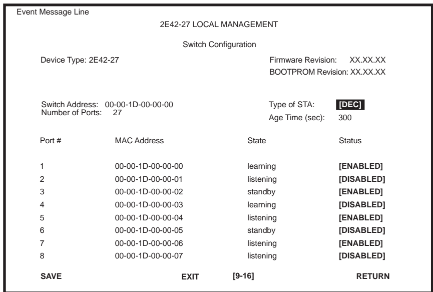
Figure 5-17 Switch Configuration Screen
