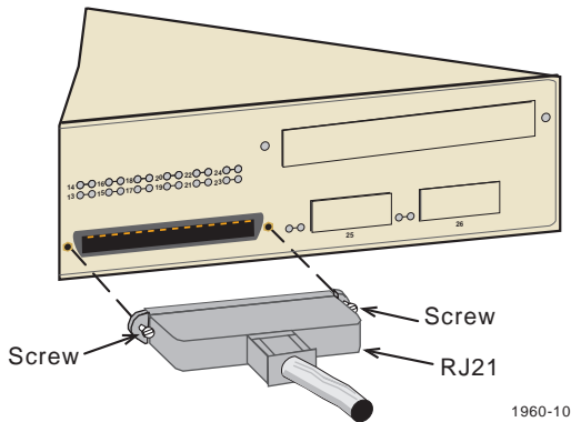
Figure 3-8 2E43-27 or 2E43-27R Straight Cable Connection
