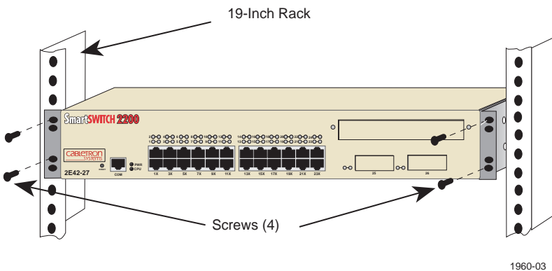
Figure 3-4 Installing the 2E4X-27 in a Rack
