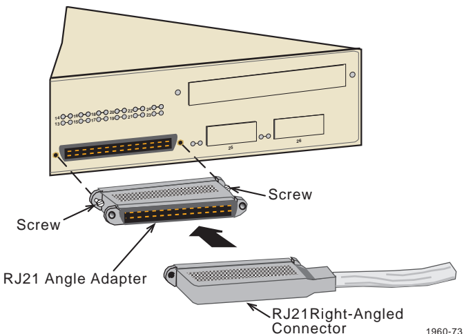
Figure 3-9 Connection Using the RJ21 Angle Adapter
