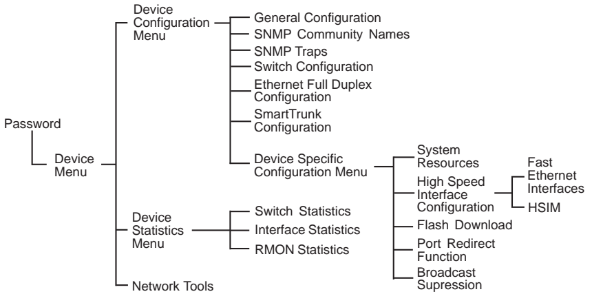
Figure 5-4 802.1D Switching Mode, LM Screen Hierarchy
