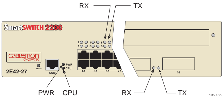
Figure 4-1 LANVIEW LEDs
