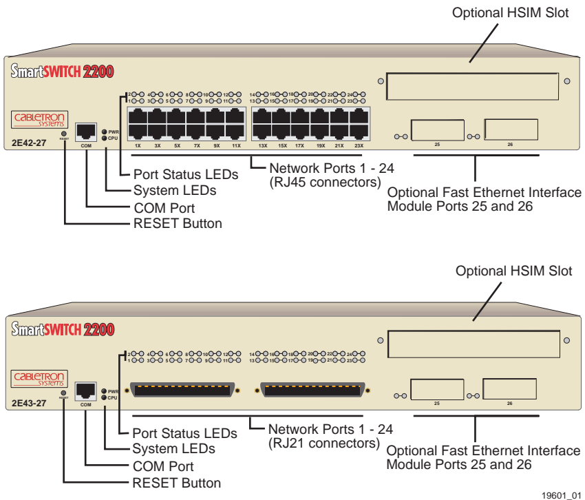
Figure 1-1 The 2E42-27 and 2E43-27
