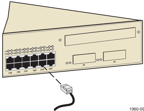
Figure 3-6 2E42-27/2E42-27R Twisted Pair Connection
