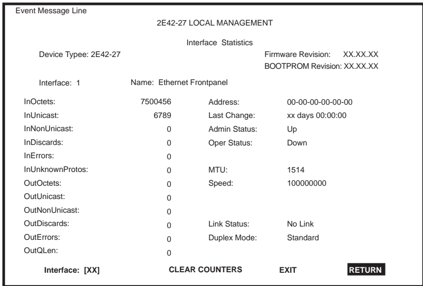
Figure 5-28 Interface Statistics Screen
