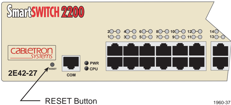
Figure 4-3 RESET Button
