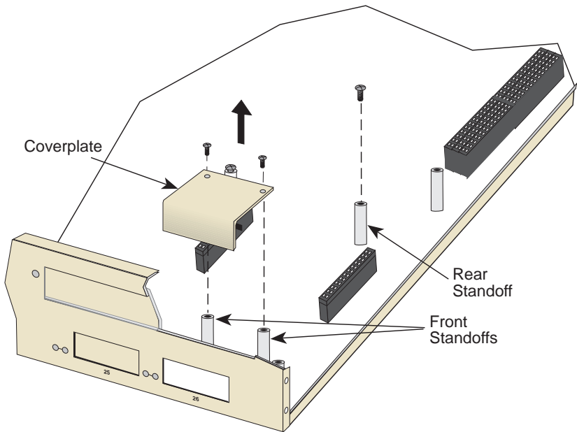
Figure C-4 Coverplate Removal
