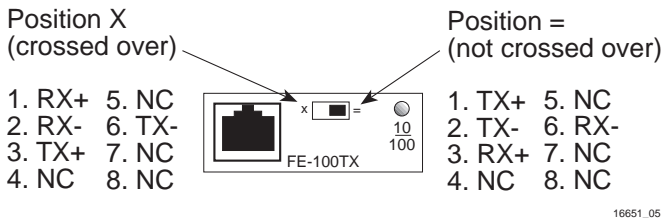
Figure 3-10 FE-100TX Crossover Switch
