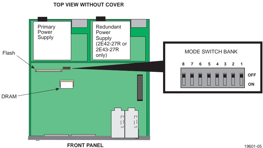
Figure C-2 2E4X-27 Mode Switch Location/Component Layout
