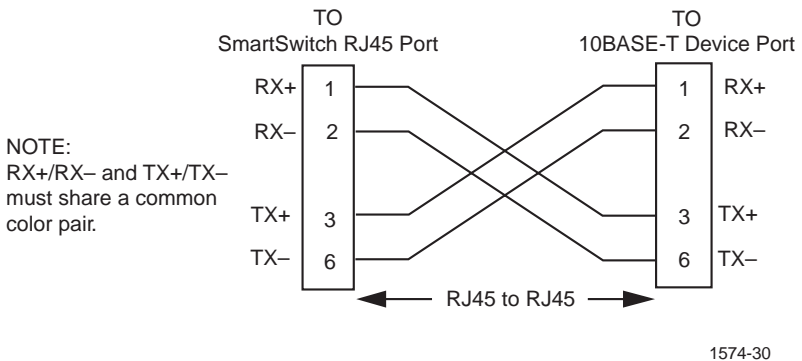
Figure 3-7 Cable Pinouts - (RJ45) Crossover Cable
