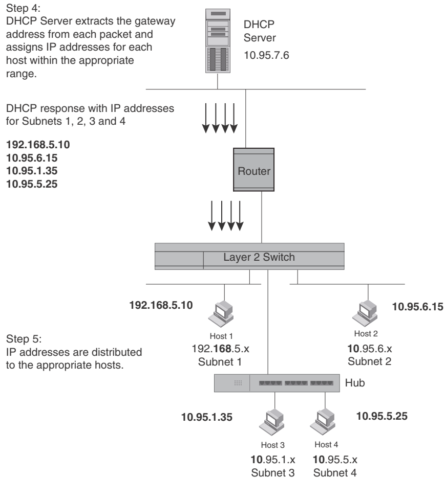
FIGURE 13 DHCP offers are forwarded back toward the requestors
