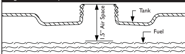
Figure 2 - Fuel Expansion
