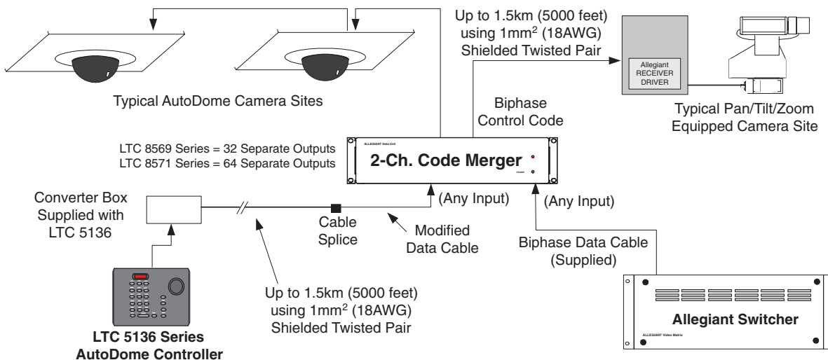
Figure 4 - AutoDome Controller Combined with Allegiant Series System
