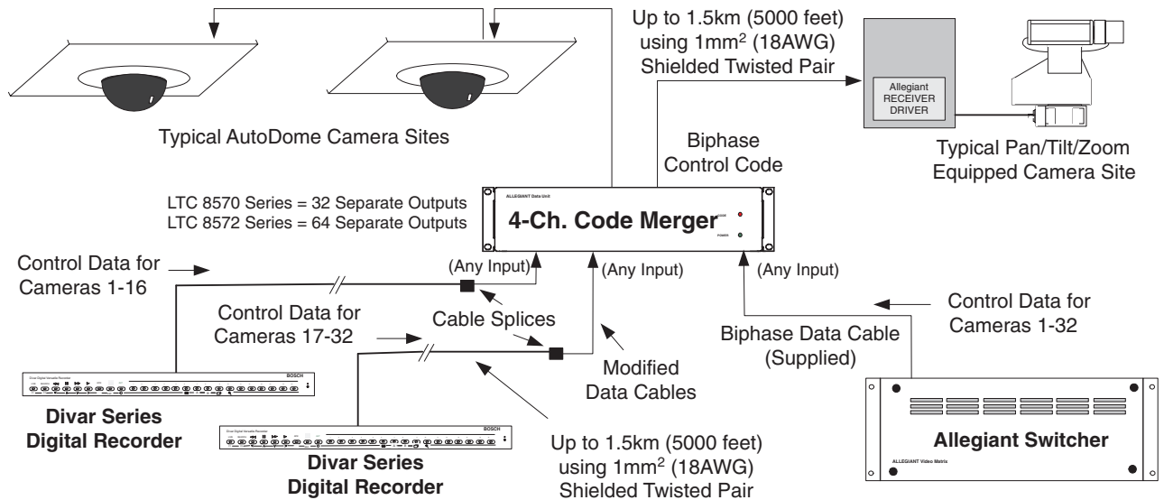
Figure 5 - Allegiant Combined with Divar Series Digital Recorders
