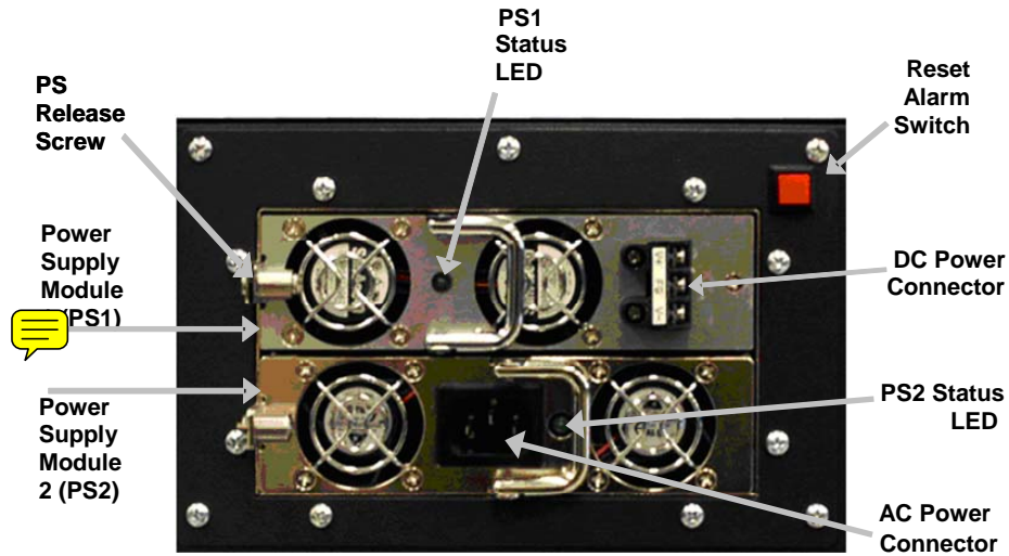
Redundant ACDC Power Supply, Close-Up
