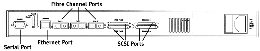
Figure 2 - Rear Panel View
