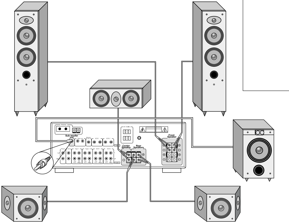
DIAGRAM 1 System Connection
