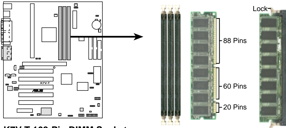
K7V-T 168-Pin DIMM Sockets
