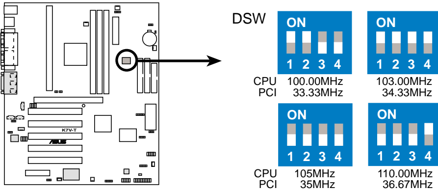
K7V-T CPU External Frequency Selection
