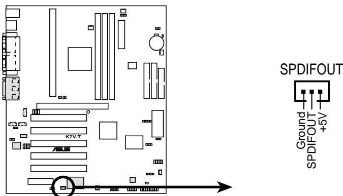
K7V-T Audio Digital Interface Connector
