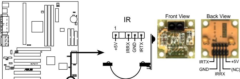
K7V-T Infrared Module Connector
