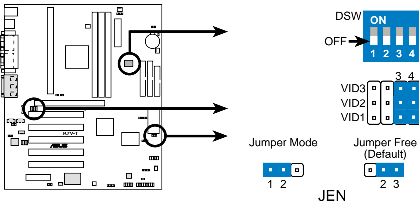
K7V-T Jumper Mode Setting
