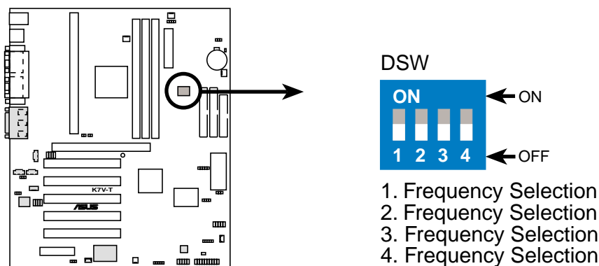
K7V-T DIP Switches
