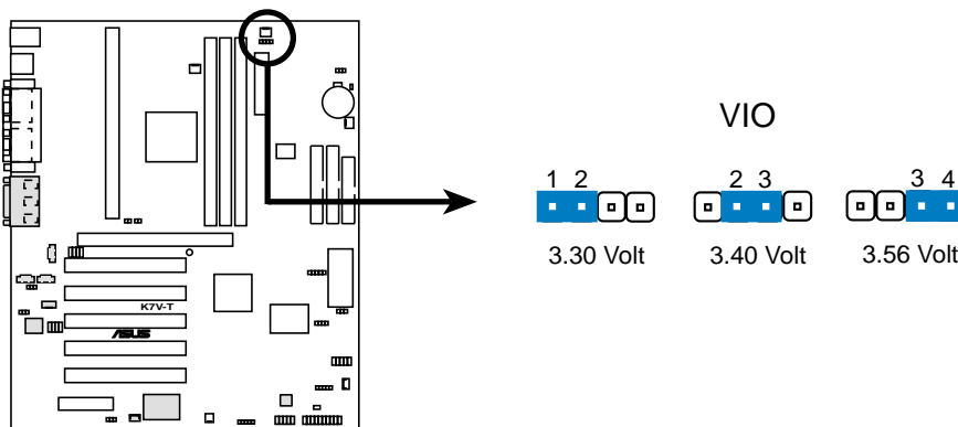
K7V-T VIO Setting
