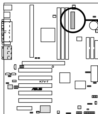
K7V-T ATX Power Connector
