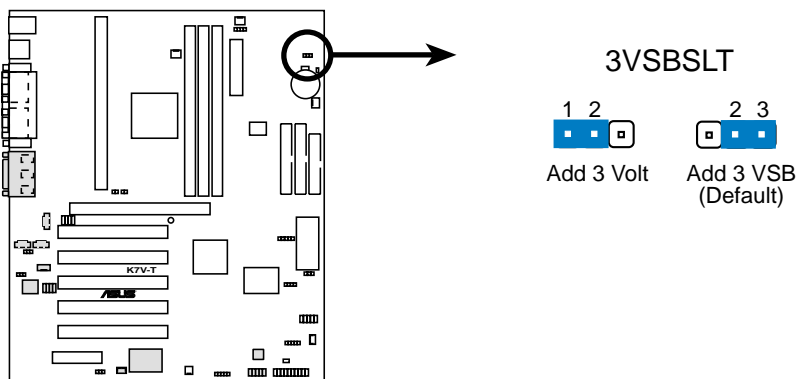
K7V-T PCI 3Volt Selection
