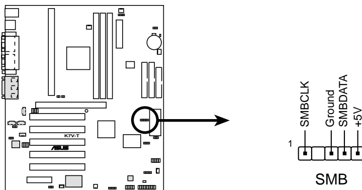
K7V-T SMBus Connector
