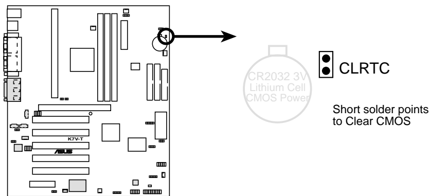
K7V-T Clear RTC RAM
