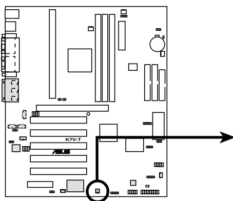
K7V-T Wake-On-Ring Connector
