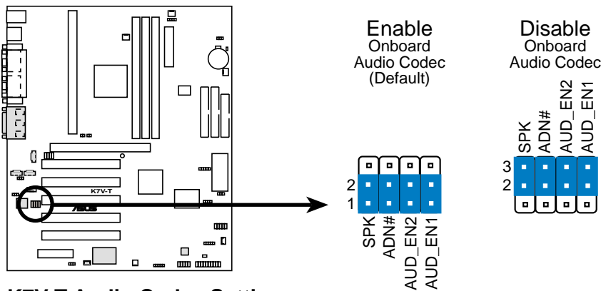
K7V-T Audio Codec Setting
