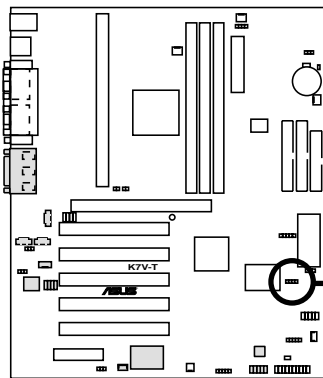
K7V-T Chassis Open Alarm Lead
