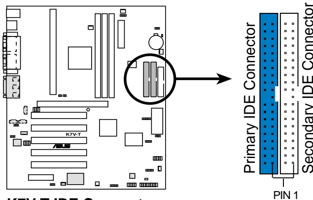
K7V-T IDE Connectors
