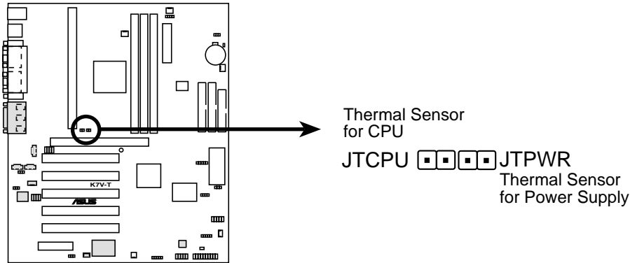
K7V-T Thermal Sensor Connectors
