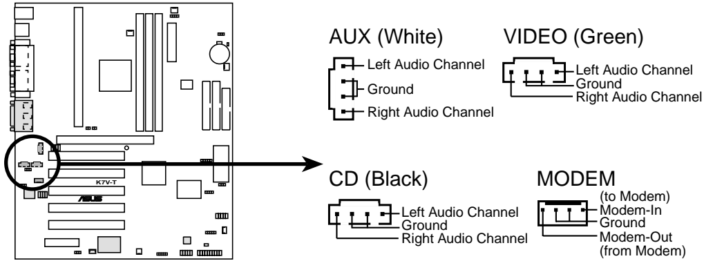
K7V-T Internal Audio Connectors
