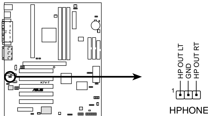
K7V-T True-Level Line Out Header
