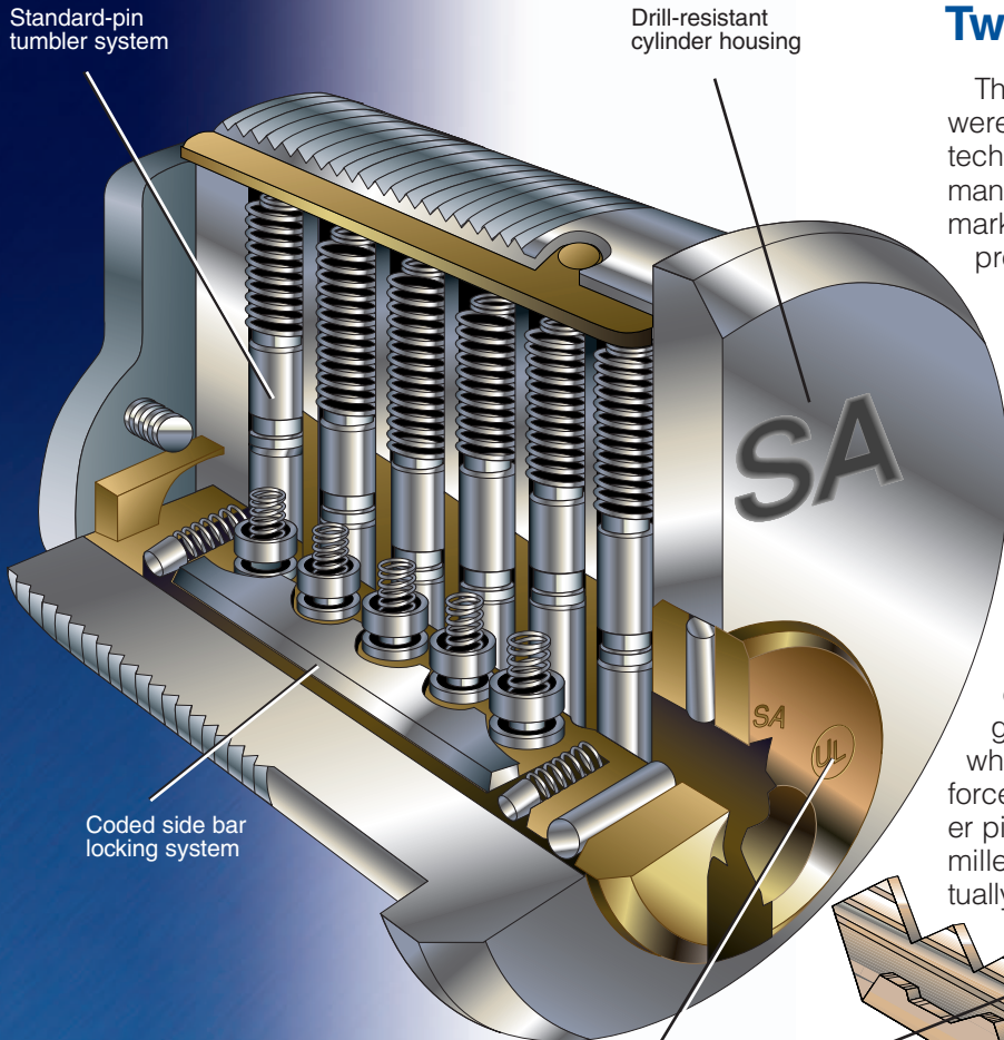
Drill-resistant cylinder plug
