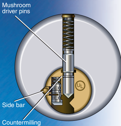
Drill-resistant cylinder plug
