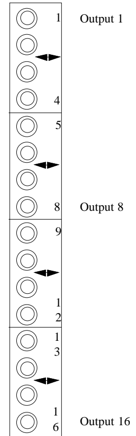
Figure 5 2010DB-11 to 2010DB- 18 Rear Panel w/ 16 BNCs Multiple-Bay System for cameras 1-256
