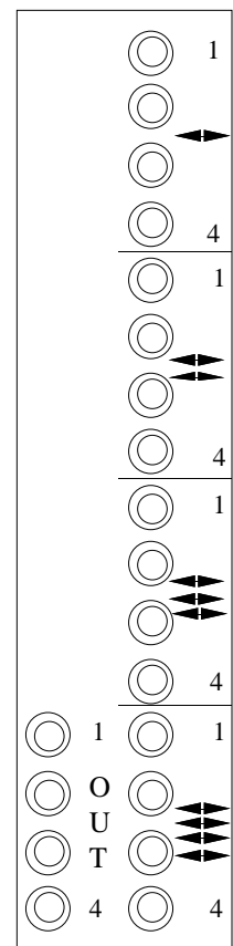
Figure 22 Video Output Module 2024VOM-2 Rear Panel
