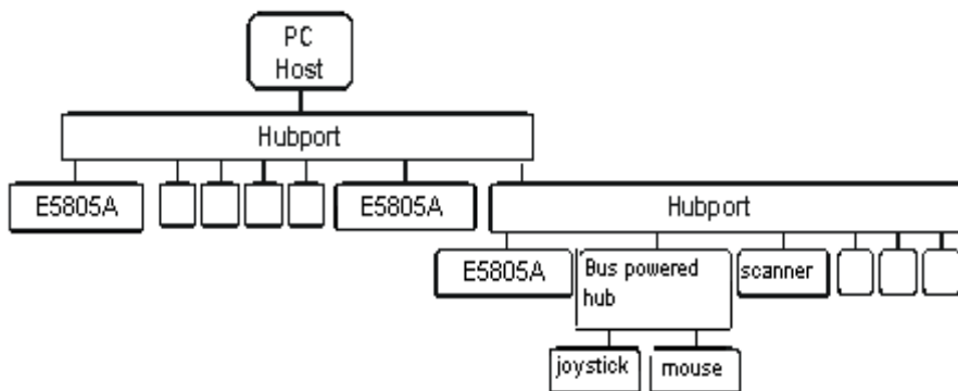
Figure 1 Hub Architecture
