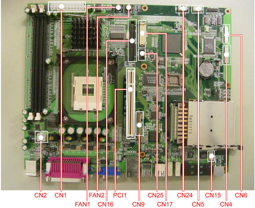
Figure 3.2: Connectors on IPPC-9151 motherboard
