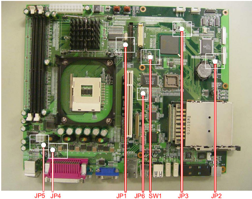
Figure 3.1: Jumpers on the IPPC-9151 motherboard
