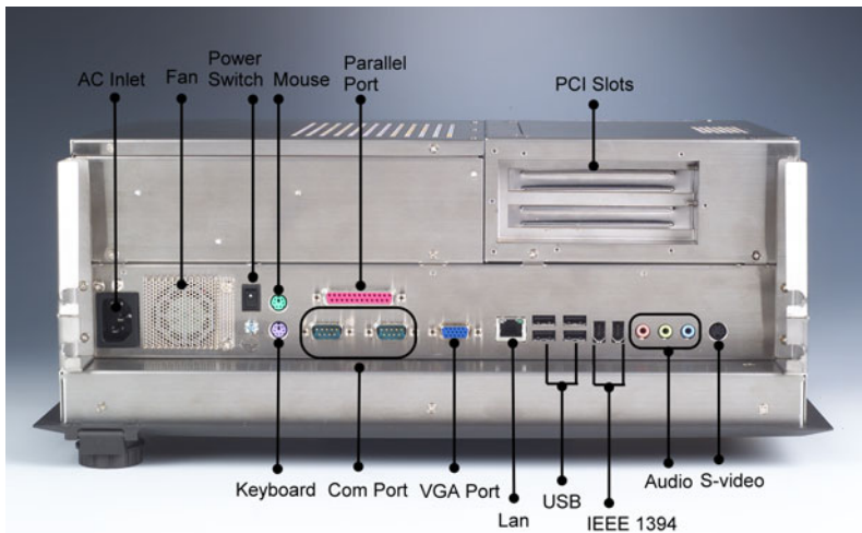
Figure 2.2: Bottom View
