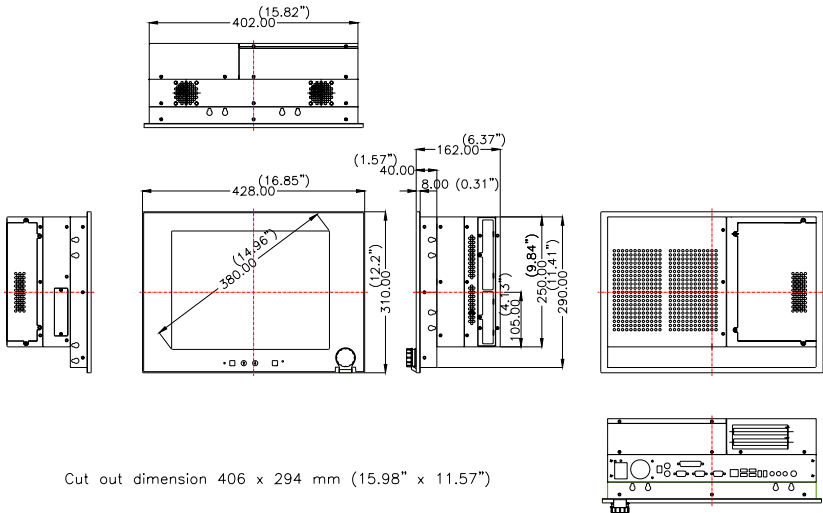
Figure 1.1: IPPC-9151FA Dimensions
