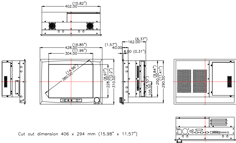
Figure 1.2: IPPC-9151GA Dimensions
