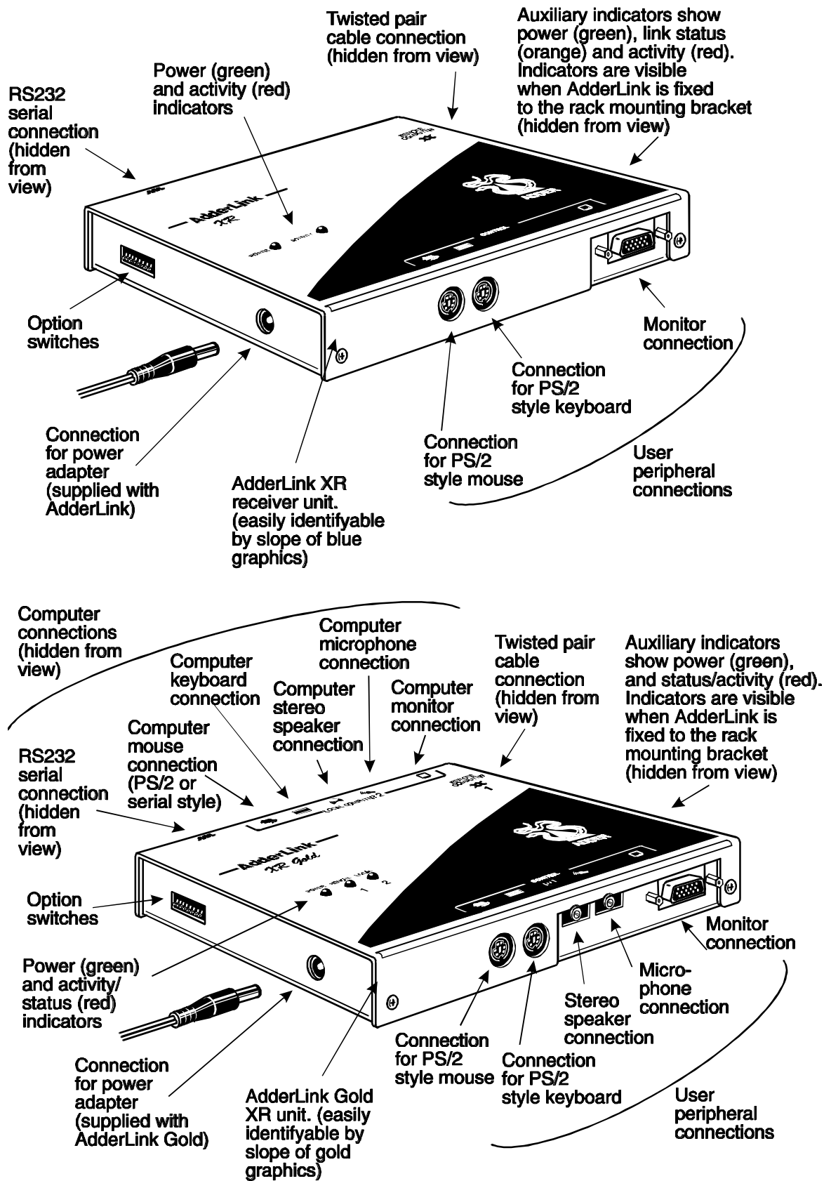
Fig. 3 - AdderLink XR (top) and AdderLink Gold (below) XR receiver units
