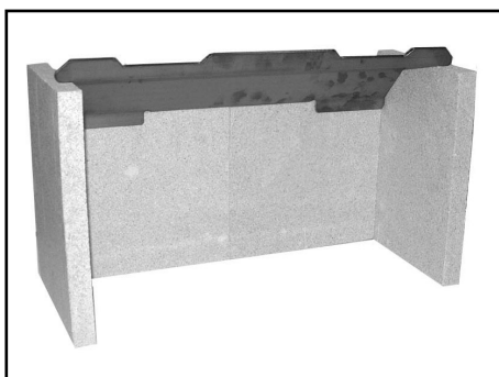
Fig. 11 Sherborne Medium Multifuel liners and throat plate.
