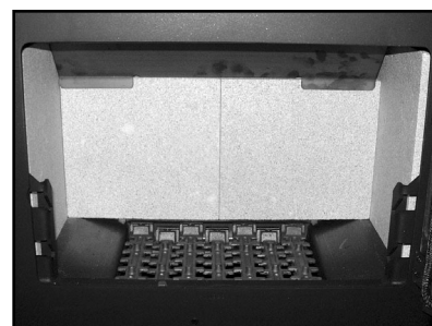
Fig. 14 Liners, throat plate and grate in Sherborne Medium multifuel.
