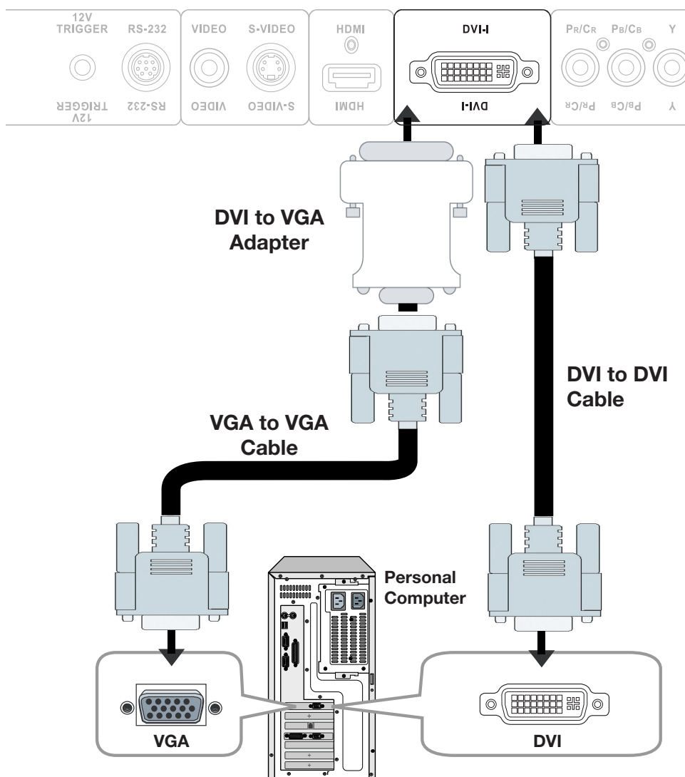
Figure 3-10. RGB Connections
