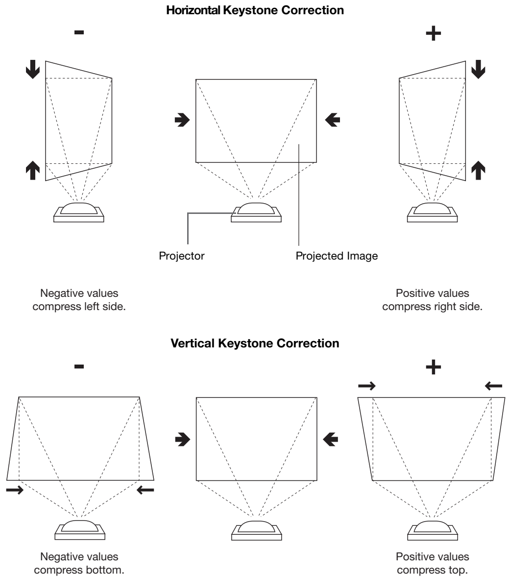
Figure 4-6. Keystone Correction
