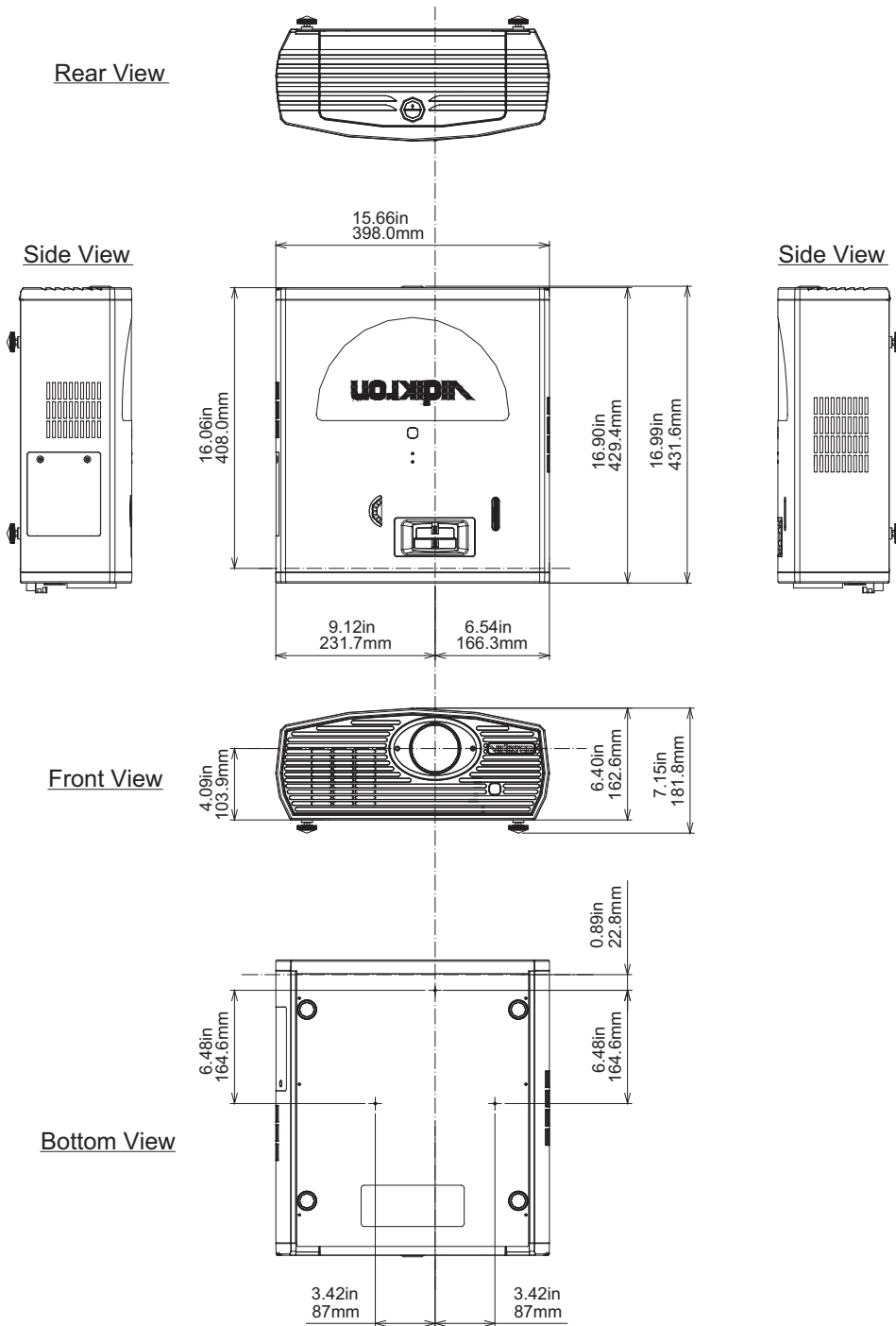
Figure 7-1. Vision 15 Dimensions
