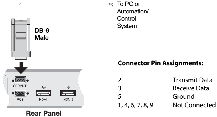
Figure 3-10. RS-232 Control System Connection
