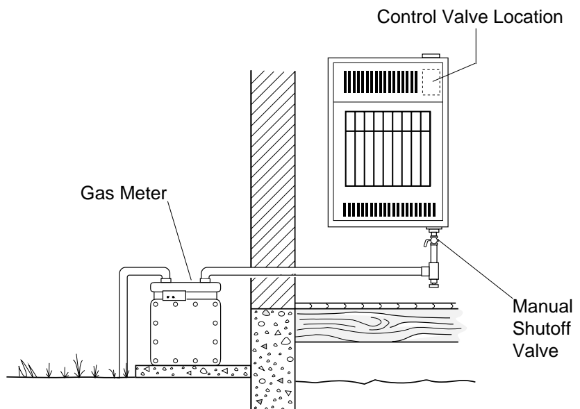
Figure 12 - Checking Gas Joints
