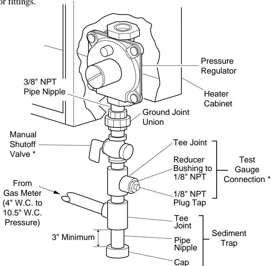
Figure 10 - Gas Connection
