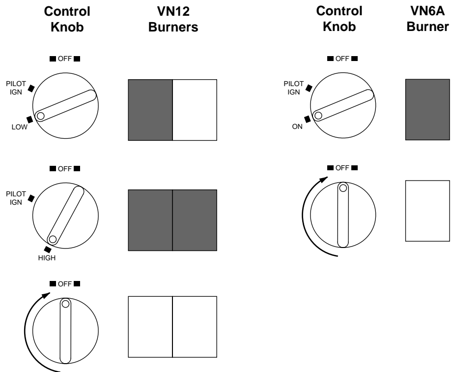
Figure 15 - Burner Patterns
