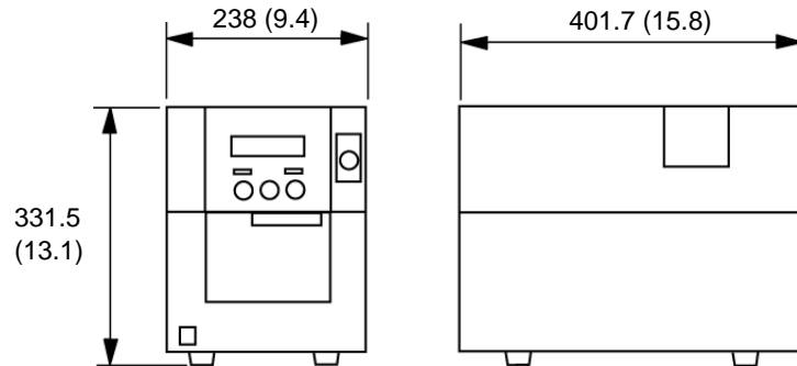
Dimensions in mm (inches)
