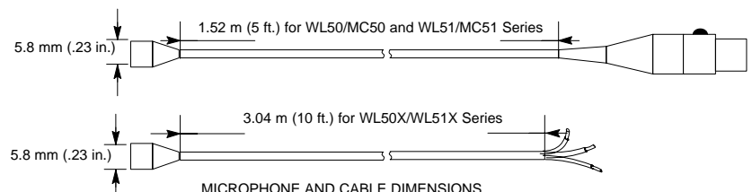
MICROPHONE AND CABLE DIMENSIONS FIGURE 3
