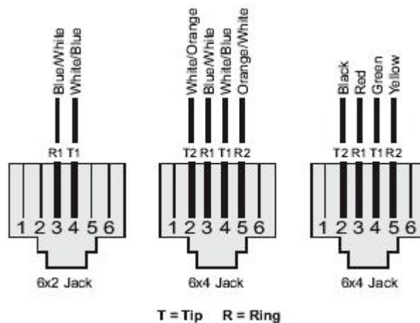
Figure C.3 - RJ-11 Pinouts
