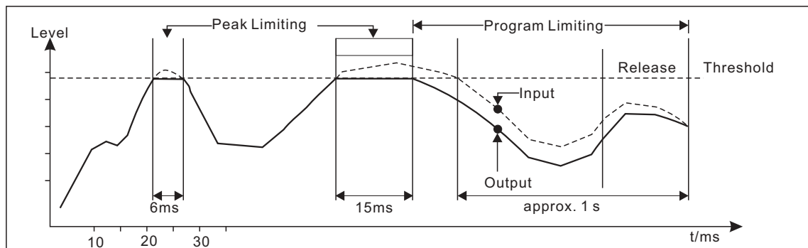
Chart. 5 SGC characteristic of the limiter section
