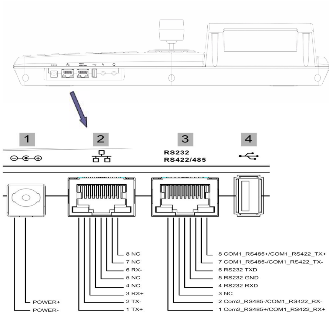
Figure 0-1 UltraKey Plus Port Connections
