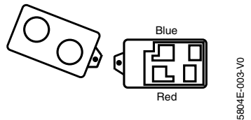
Figure 3: 5804E shown open, buttons facing down
