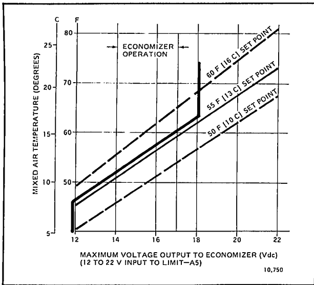
FIG. 4—ECONOMIZER/MIXED AIR LOW LIMIT—MAXIMUM VOLTAGE OUTPUT.
