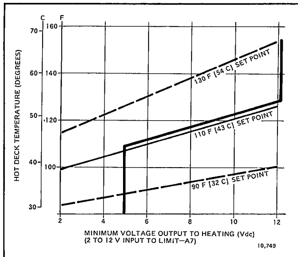
FIG. 6—HOT DECK LIMIT—MINIMUM VOLTAGE OUTPUT.
