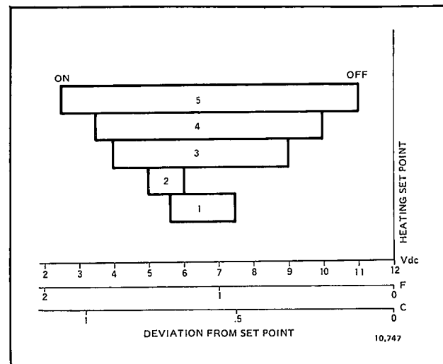
FIG. 8—W7083A ELECTRIC HEAT SEQUENCER STAGE ON-OFF AND OVERLAP.
