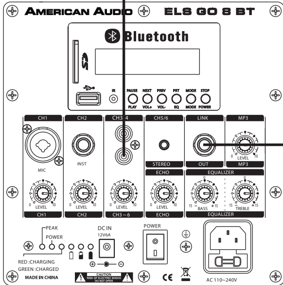
1/4" TRS-RCA Line Level Cable
